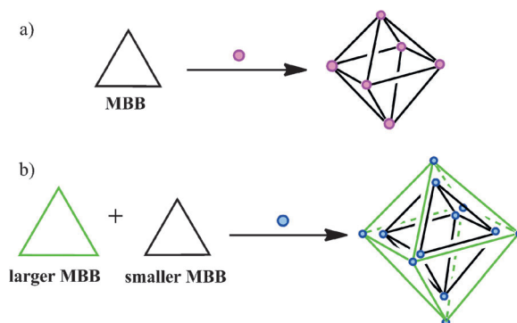
Scheme 1. The rational design of double-walled octahedra by means of two C_3 -symmetric trigonal MBBs.
